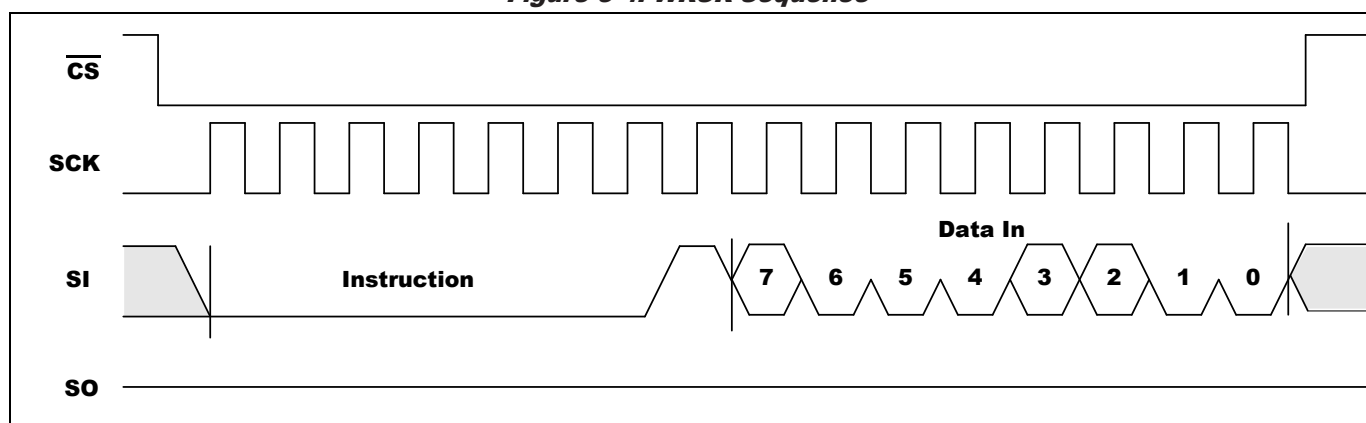
Figure 5-4. WRSR Sequence
