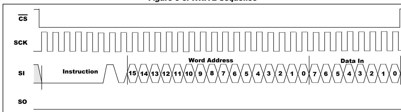
Figure 5-6. WRITE Sequence
