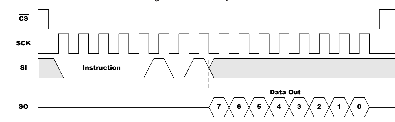
Figure 5-3. RDSR Sequence
