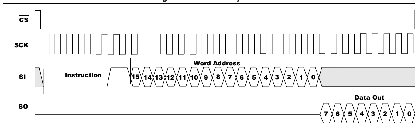
Figure 5-5. READ Sequence
