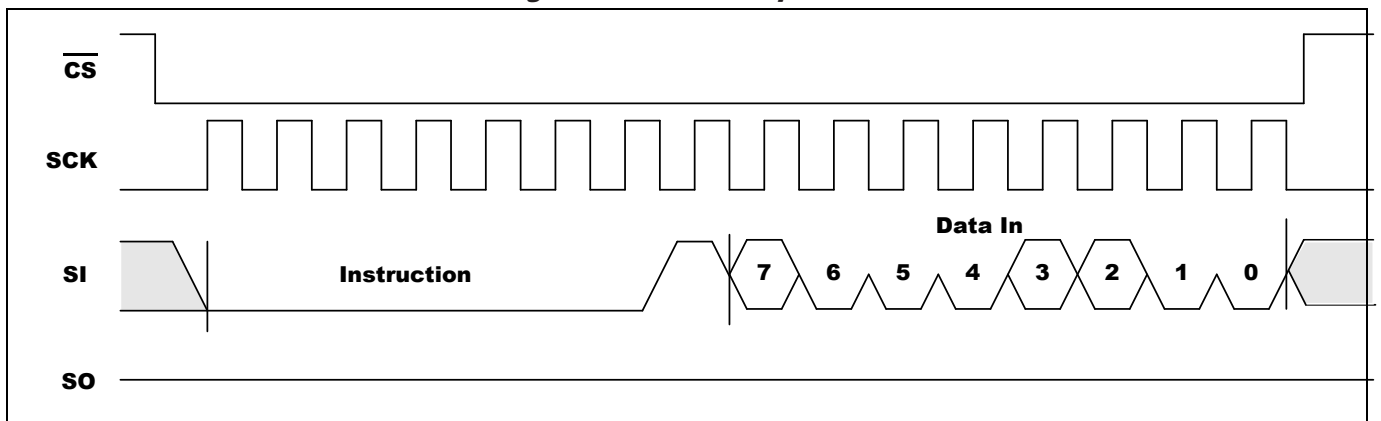
Figure 5-4. WRSR Sequence
